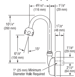
ETF-500-S-H with Surgical Bend Spout and Shower Spray Head
